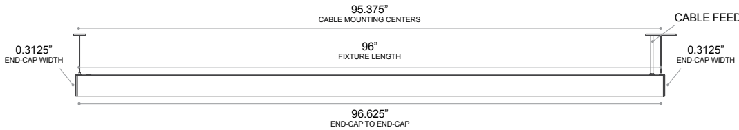
8' FIXTURE
