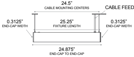
2' FIXTURE
