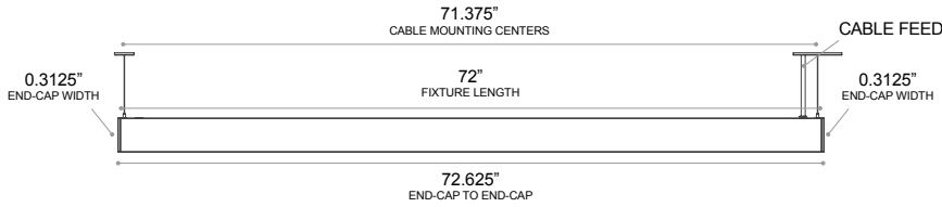
6' FIXTURE
