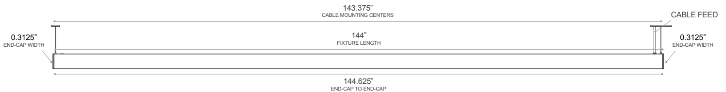
12' FIXTURE
