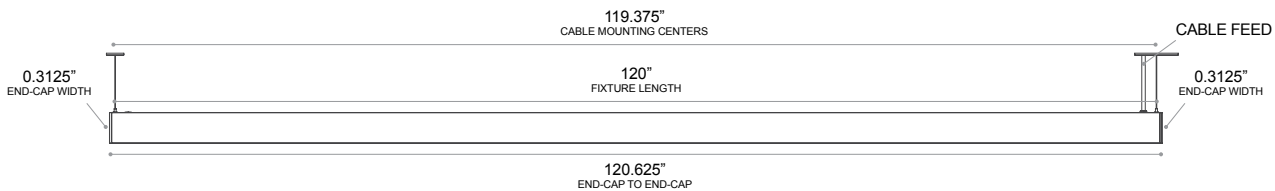
10' FIXTURE
