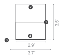
CROSS-SECTION: WW
